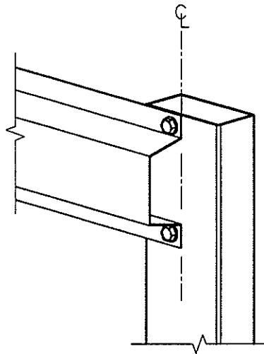
VIEW A
